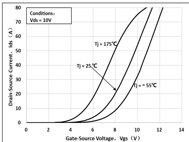
Fig 6: Transfer Characteristic
