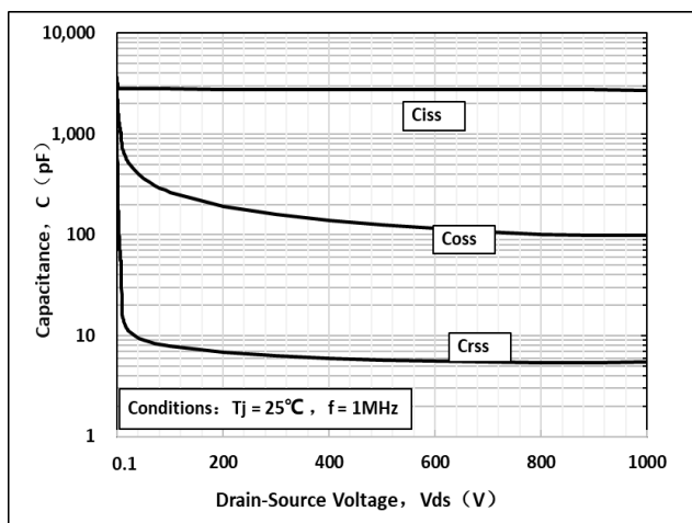
Fig 17: Capacitance Characteristics
