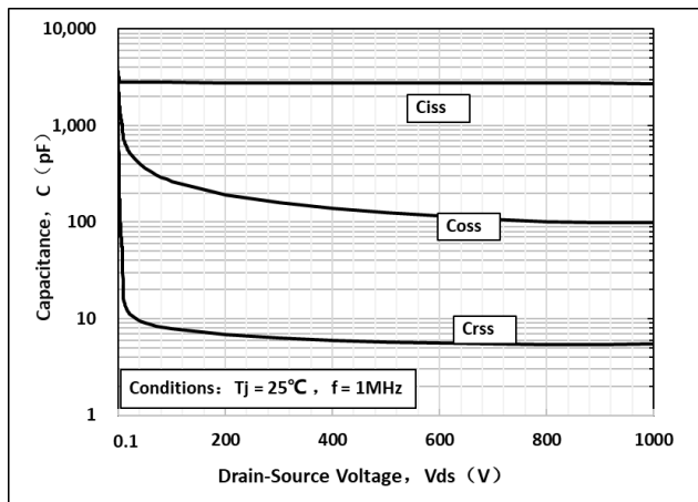
Fig 17: Capacitance Characteristics
