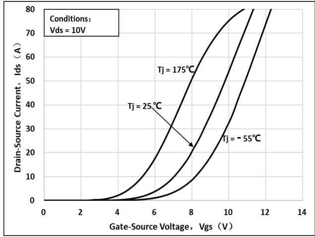
Fig 6: Transfer Characteristic
