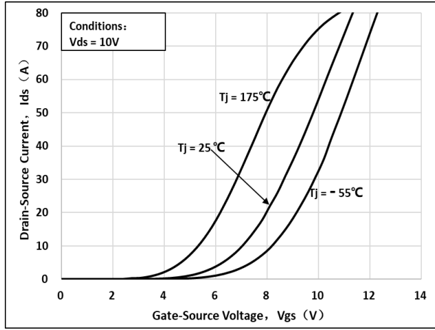
Fig 6: Transfer Characteristic
