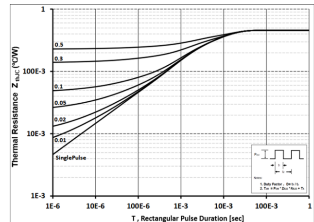
Fig 18: Transient Thermal Impedance
