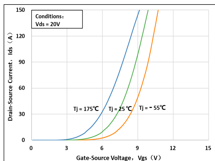
Fig 6: Transfer Characteristic
