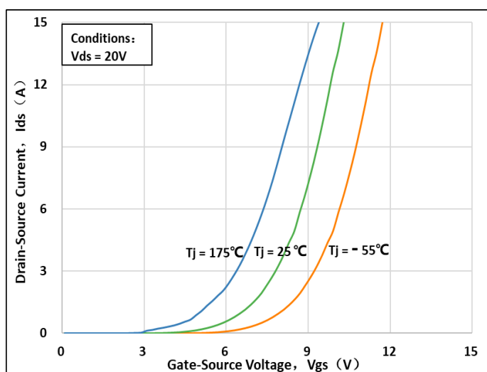
Fig 6: Transfer Characteristic
