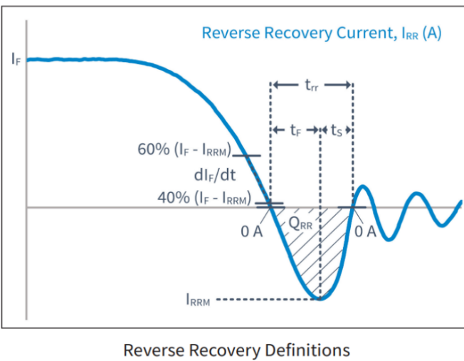
Figure C. Definition of body diodeswitching characteristics
