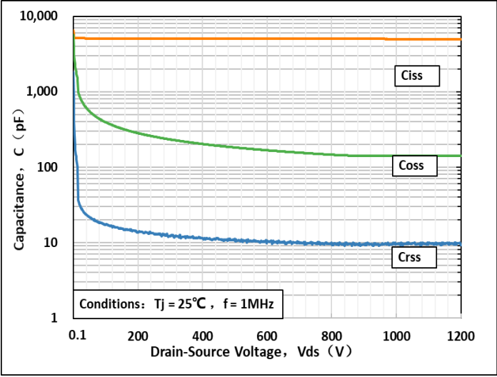
Fig 17: Capacitance Characteristics
