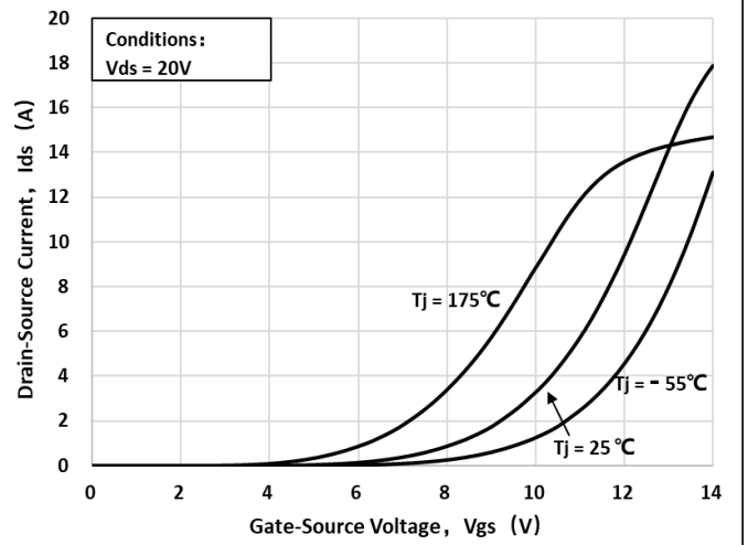
Fig 6: Transfer Characteristic
