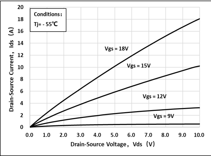
Fig 1. Output Characteristic (T J =-55°C)
