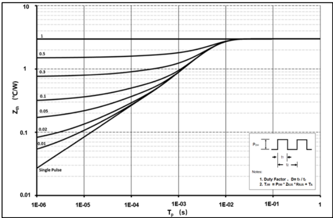
Fig 17: Transient Thermal Impedance
