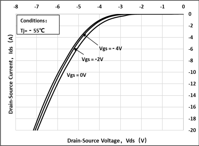
Fig 7: Body-diode Characteristic (T J =-55°C)
