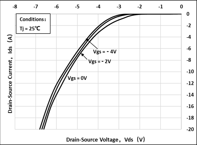
Fig 8: Body-diode Characteristic (T J =25°C)
