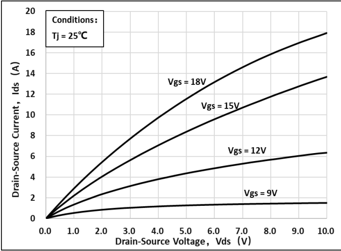
Fig 2. Output Characteristic (T J =25°C)
