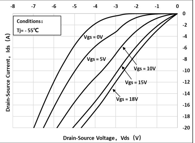
Fig 12: 3rd Quadrant Characteristic(T J =-55°C)
