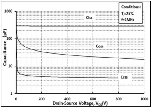
Fig 15: Capacitance Characteristic
