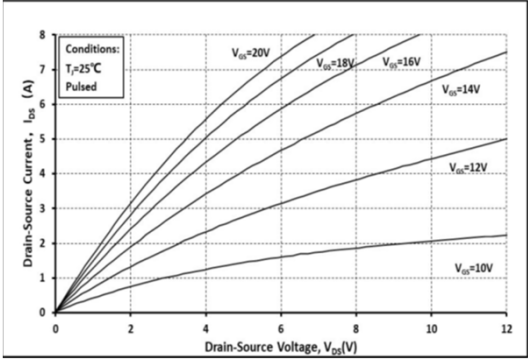
Fig 2. Output Characteristic (T J =25°C)
