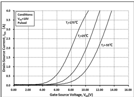
Fig 6: Transfer Characteristic
