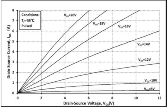
Fig 1. Output Characteristic (T J =-55°C)
