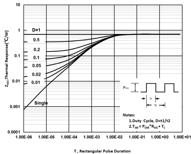
Fig 8: Transient Thermal Impandance
