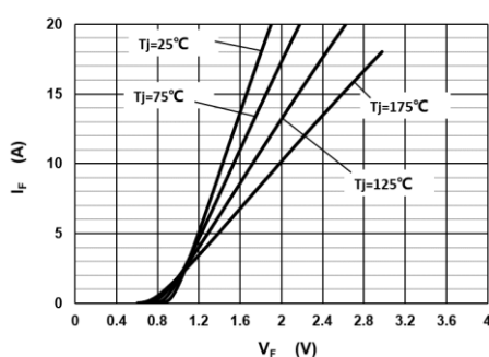
Fig 1: Forward Characteristics
