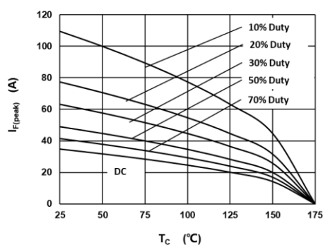
Fig 3: Current Derating
