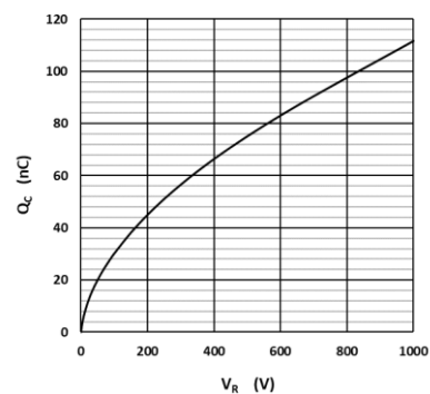
Fig 6: Reverse Charge vs. Reverse Voltage
