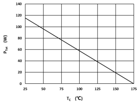
Fig 4: Power Derating
