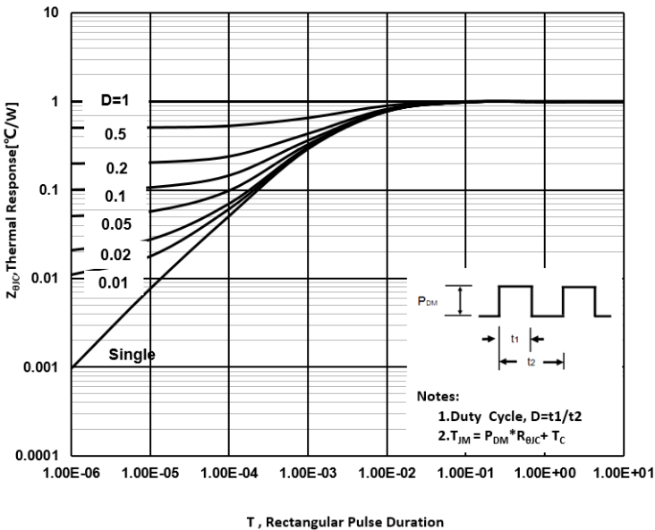
Fig 8: Transient Thermal Impandance
