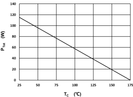
Fig 4: Power Derating
