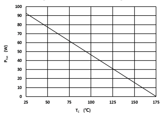
Fig 4: Power Derating
