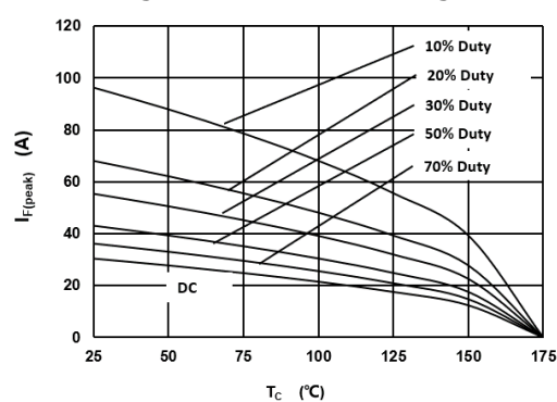
Fig 3: Current Derating
