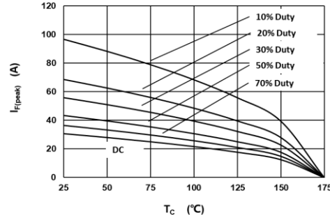
Fig 3: Current Derating
