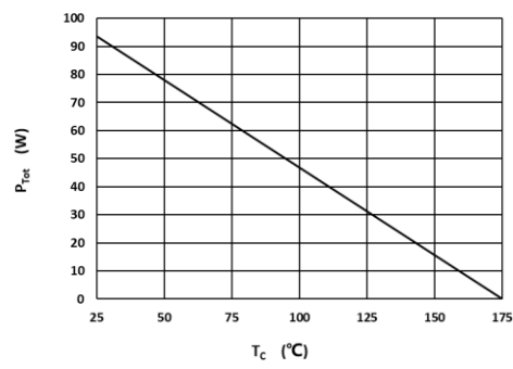
Fig 4: Power Derating
