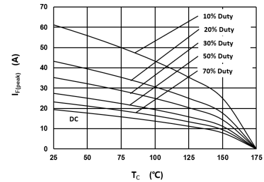
Fig 3: Current Derating
