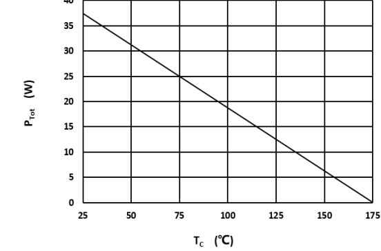
Fig 4: Power Derating
