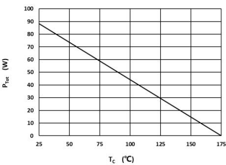
Fig 4: Power Derating
