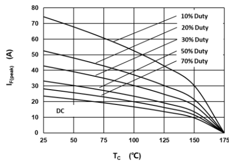
Fig 3: Current Derating
