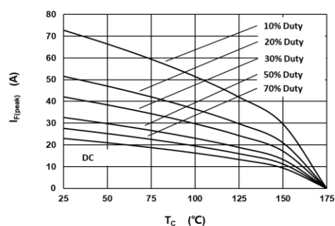
Fig 3: Current Derating
