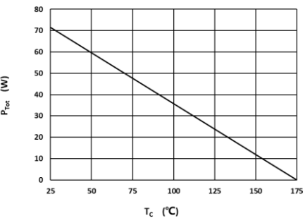
Fig 4: Power Derating
