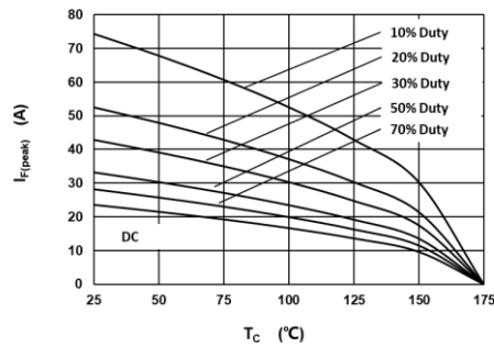
Fig 3: Current Derating
