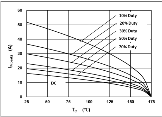
Fig 3: Current Derating
