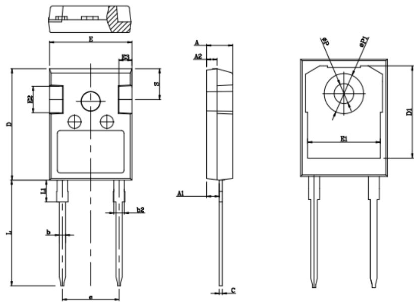
COMMON DIMENSIONS
