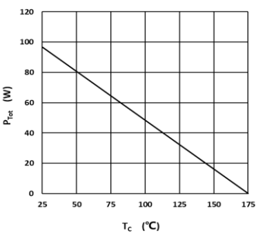
Fig 4: Power Derating
