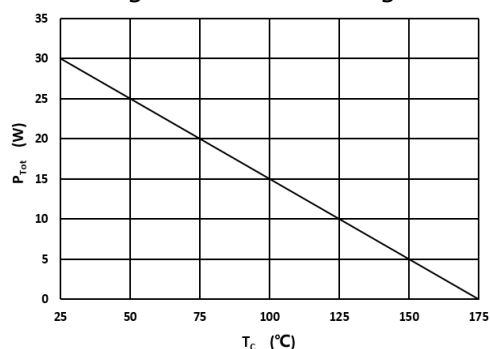
Fig 4: Power Derating
