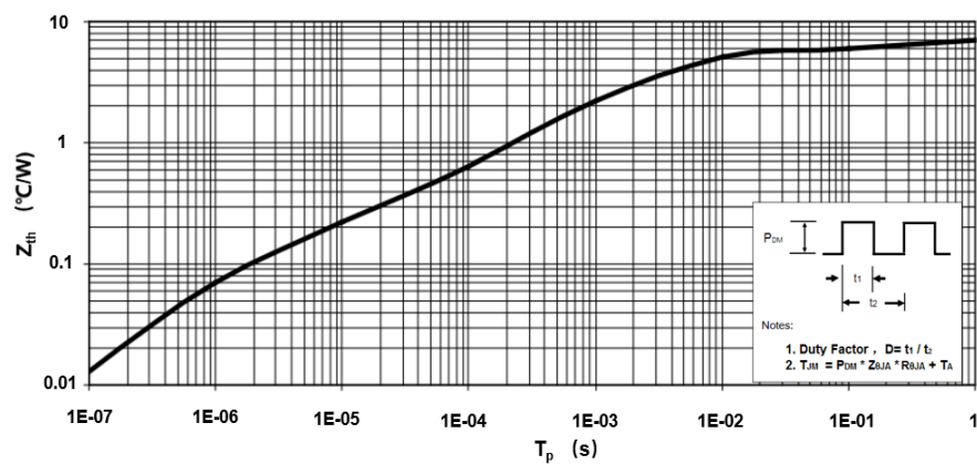
Fig 8: Transient Thermal Impandance
