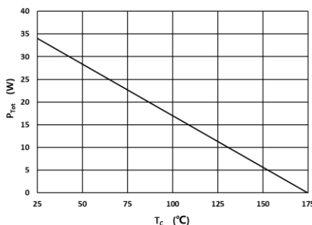
Fig 4: Power Derating
