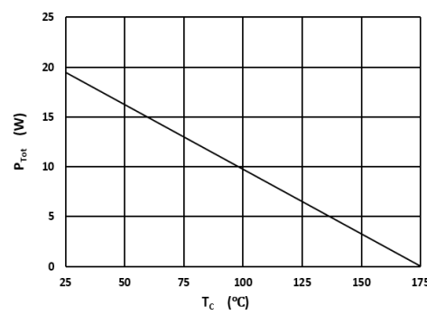
Fig 4: Power Derating
