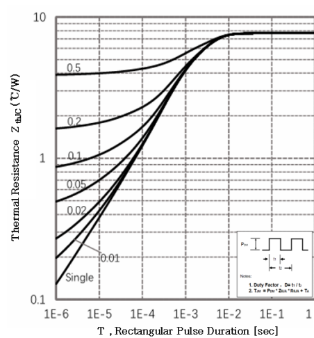
Fig 8: Transient Thermal Impedance
