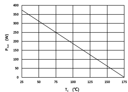
Fig 4: Power Derating
