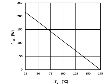
Fig 4: Power Derating
