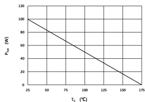
Fig 4: Power Derating
