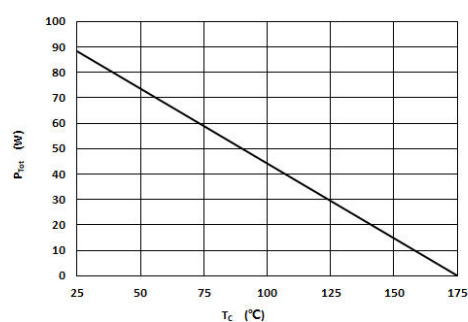
Fig 4: Power Derating
