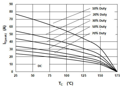
Fig 3: Current Derating
