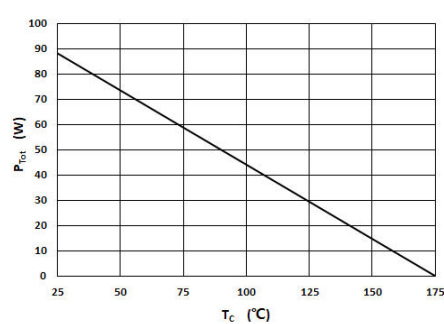
Fig 4: Power Derating
