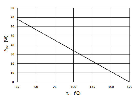
Fig 4: Power Derating
