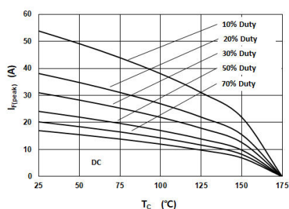
Fig 3: Current Derating
