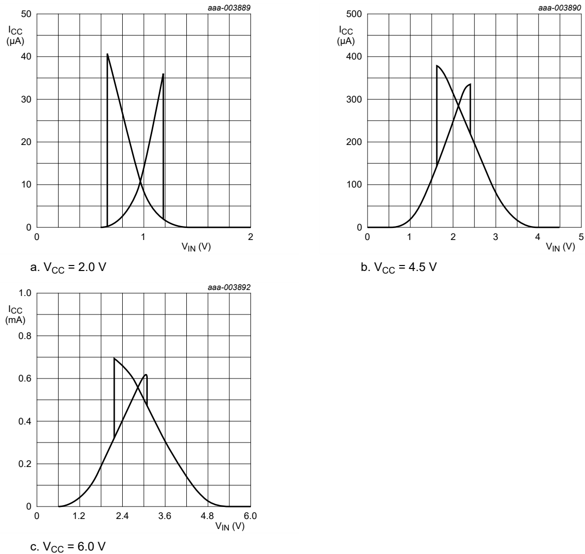
Fig. 8. Typical 74HC132 transfer characteristics
