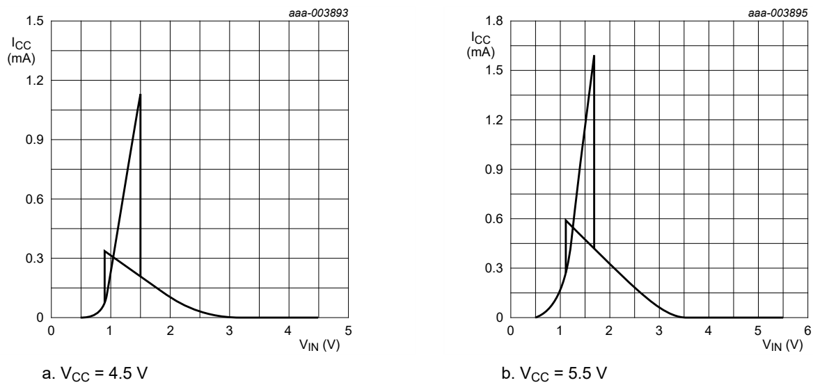
Fig. 9. Typical 74HCT132 transfer characteristics
