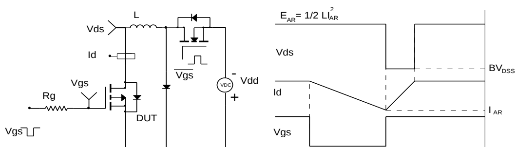
Figure 3: Unclamped Inductive Switching Test Circuit &amp; Waveform
