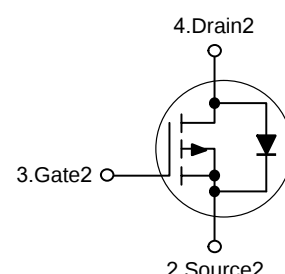
P-Channel
