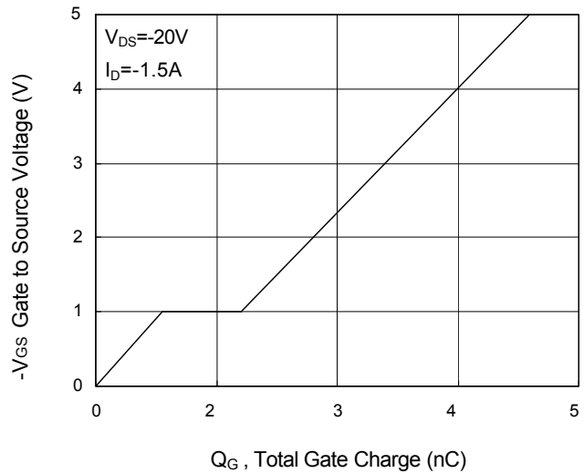
Fig.4 Gate-Charge Characteristics
