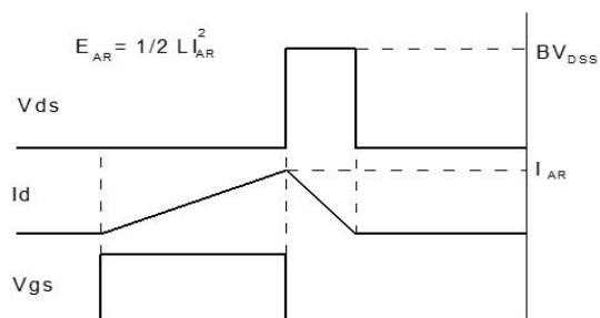
Figure 3: Unclamped Inductive Switching Test Circuit &amp; Waveform
