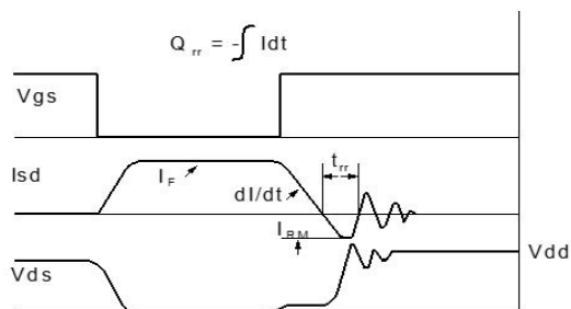
Figure 4: Diode Recovery Test Circuit &amp; Waveform
