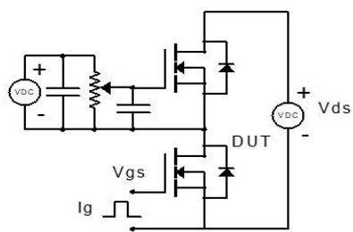
Figure 1: Gate Charge Test Circuit &amp; Waveform
