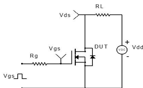
Figure 2: Resistive Switching Test Circuit &amp; Waveform
