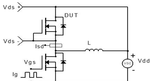
Figure 4: Diode Recovery Test Circuit &amp; Waveform
