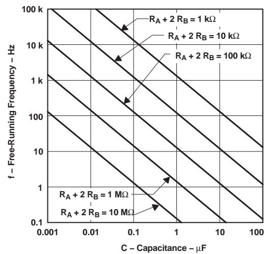
Figure 14. Free-Running Frequency
