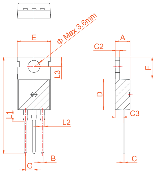
TO-220C
