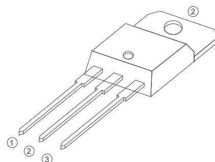
TO-220A Insulated
