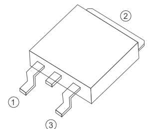
TO-252
