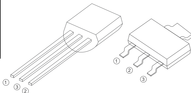
TO-92
